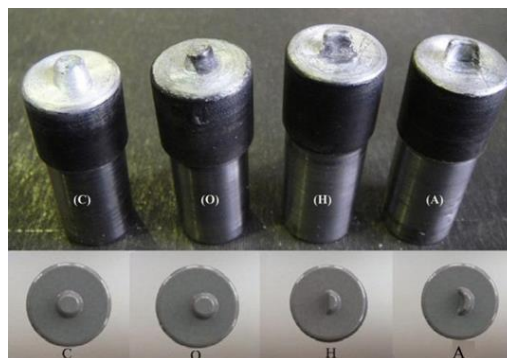
Fig 6 Different tool pins and their positions
