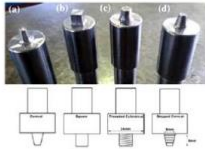
Fig. 4 Different pin profiles. a Conical b Square. c Threaded
