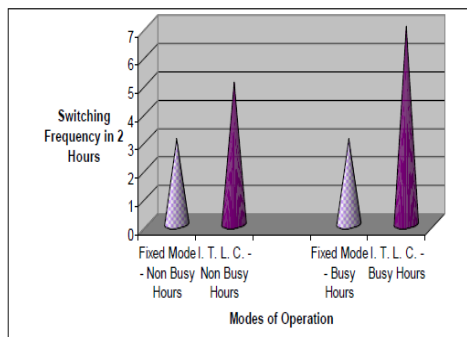
Figure 5: Switching Frequency of Green Signal for 2 Hours Duration
