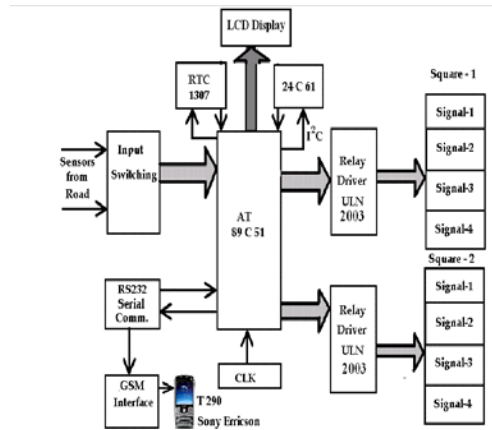
Figure 2: Block Schematic of Intelligent Traffic Light Controller with GSM Interface.
