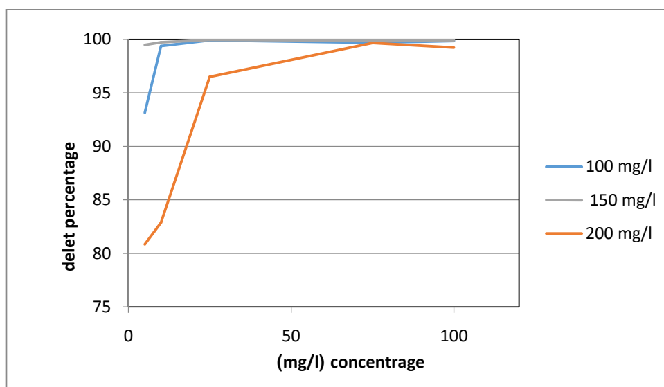
Figure 6. Effect of different concentrations on perictal removal at different load inlet to BOD in the reactor in a continuous aeration reactor suspended growth (during hydraulic retention time 2 hours)
