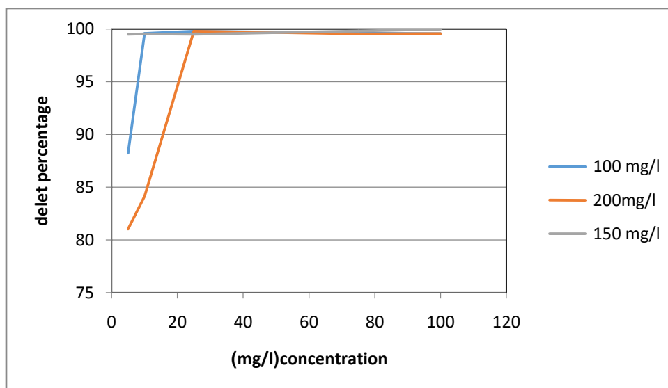
Figure 7. Effect of different concentrations on perictal removal at different load inlet to BOD in the reactor in the continuous aeration reactor suspended growth (during hydraulic retention time 5 hours
