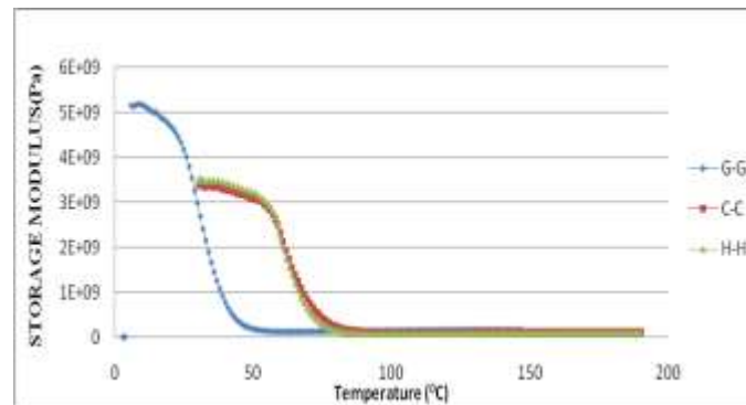
Fig: 15. (10 Hz) storage modulus Vs Temperature
