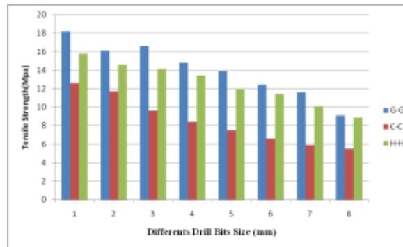
Fig:9 Open Hole Tensile Strength
