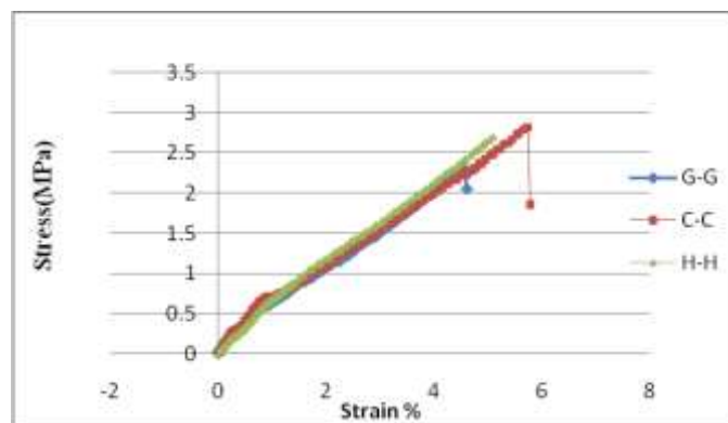
Fig: 8 Comparisons of Stress Strain Curves
