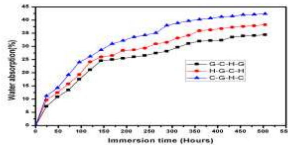
Fig:3. Water absorption
