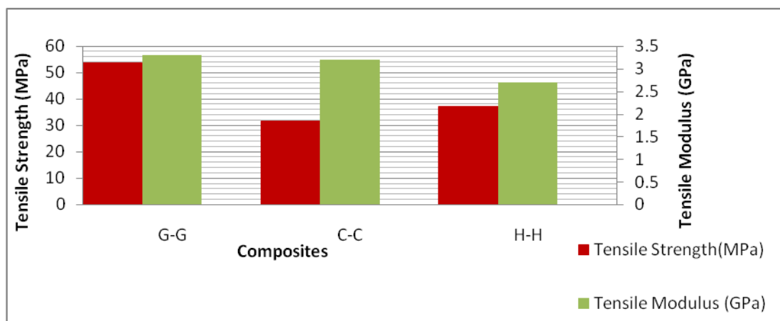
Fig: 7 Comparisons of Tensile Strength and Tensile Modulus
