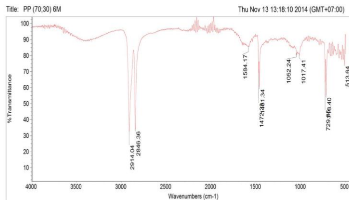
Figure 4: ‘Spektrum of FT-IR composite from PP-EFB rasio 70:30 with fiber size 63 \mu\text{m} ’
