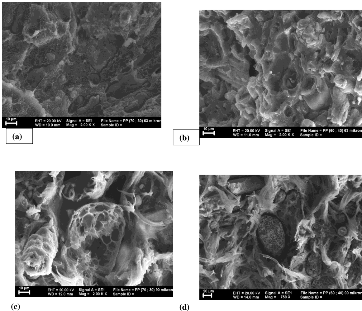
Figure 3: 'Morphology analysis with SEM composite PP: fiber, (a). (70:30), (b). (60:40) filler size 63 \mu\text{m} and (c). (70:30), (d). (60:40) filler size 90 \mu\text{m} '
